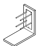
Elle Bottle design: Ronda Design Lab L 300 H 300 P 150 mm
