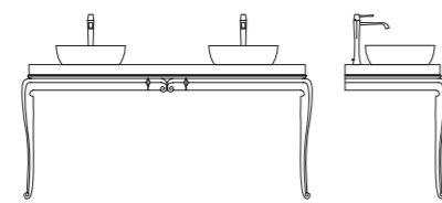
AB 412 mobile bagno bathroom furniture cm 168x59xh78h
