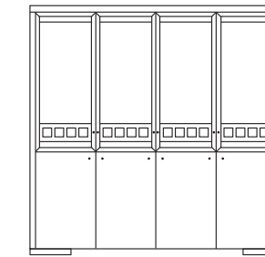
VVT 69 Vetrina 4 ante 4 doors glasscupboard cm 189 x 47 h 215
